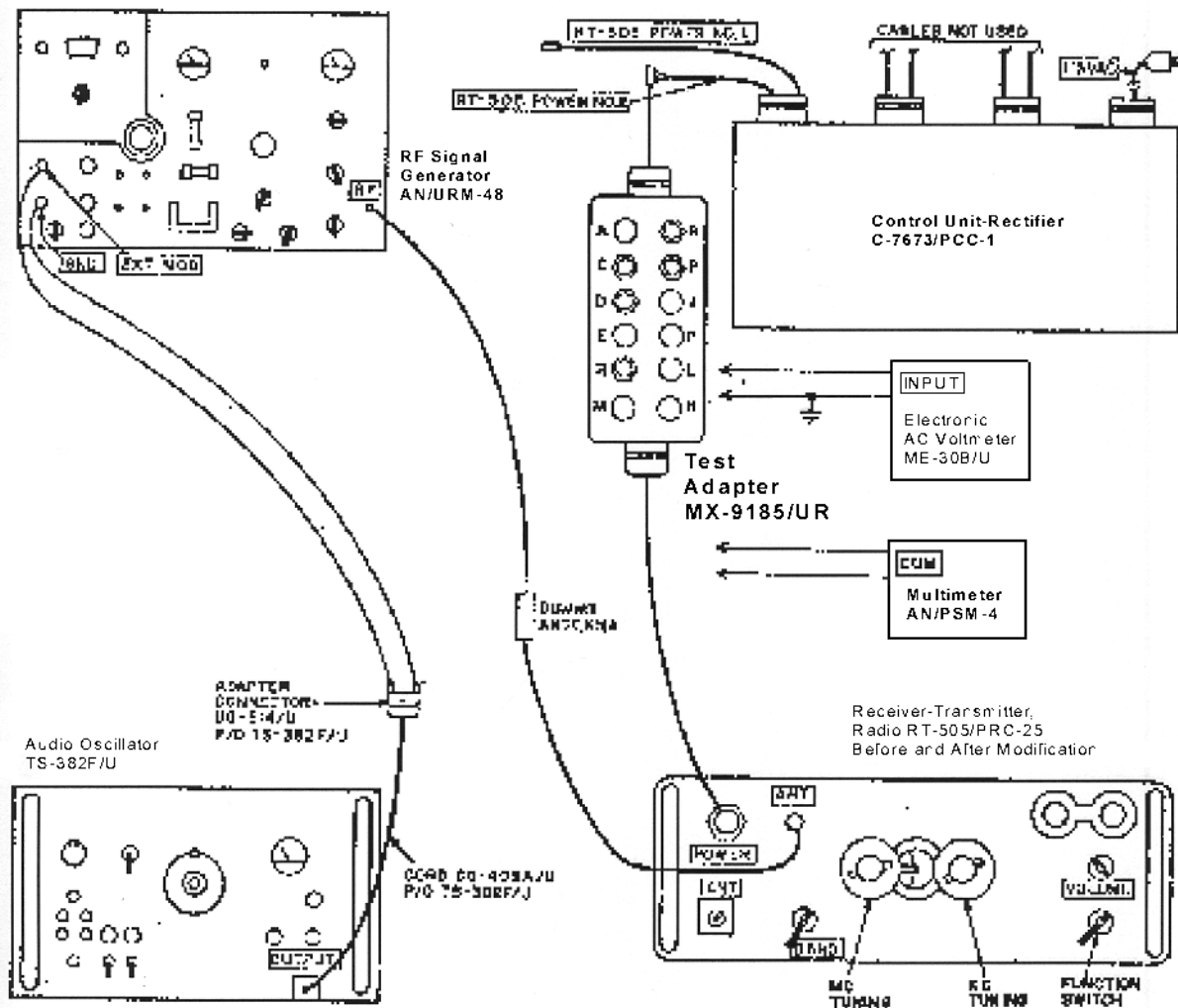
Figure 1. Receiver-Transmitter, RT-505/PRC-25, Test Setup
