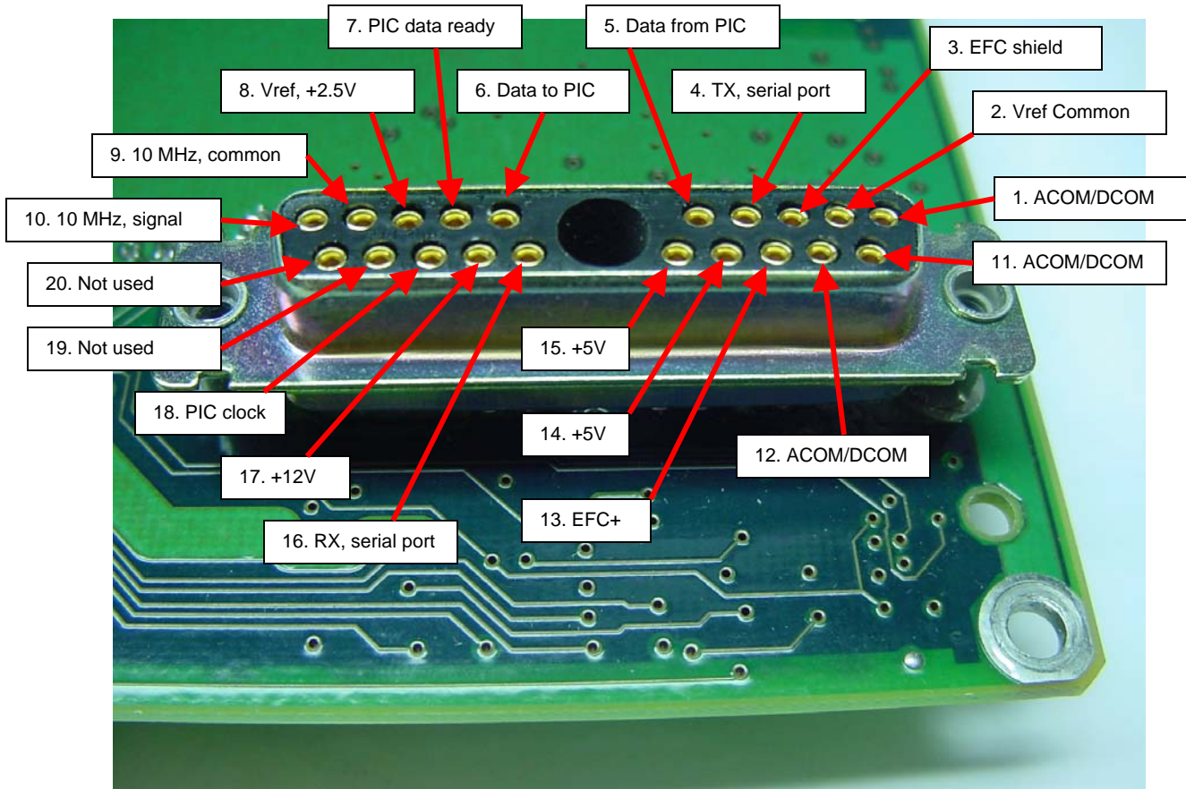
Figure 2. D-sub with coax insert on circuit side of PCB.
