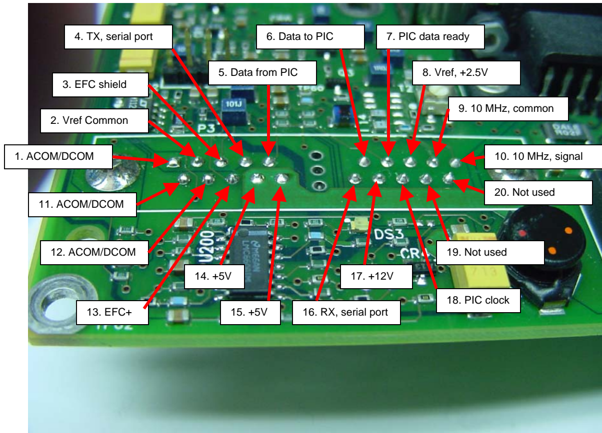
Figure 1. Component side of E1938A controller board.
